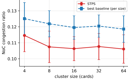
Figure 10: NoC congestion ratio versus cluster size (bursty arrivals, task count scaled with cards, 5 seeds, 95 % CI). STPS stays below the best baseline from 4 to 64 cards, holding a stable 8–12% relative advantage.
